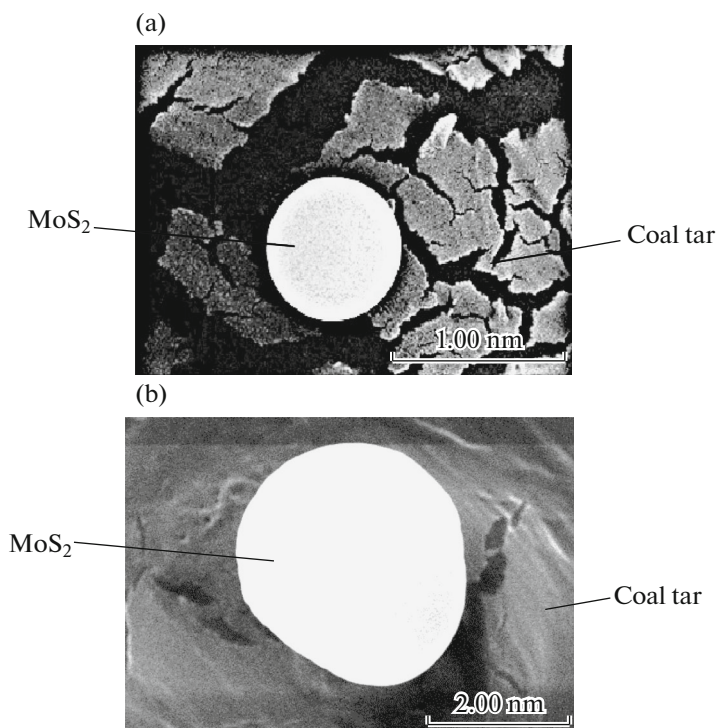
Fig. 2. Electron-microscopic images of the formation of MoS 2 particles (globules) with diameters of (a) 500 and (b) 1000 nm in the coal tar.
